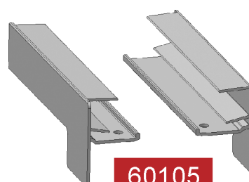
Adjoining frame bottom 105mm Dyed in all colors
