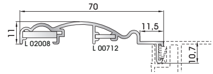
Hooked casing trim "Flat"
