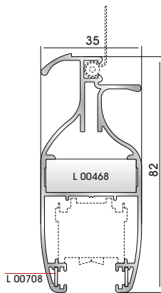
94505 W=1028gr/m A=0,434m 2 /m Insect screen sash
