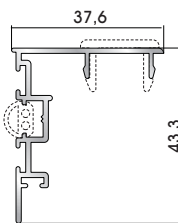
94042 W=426gr/m A=0,252m 2 /m Hook (for 94505, insect screen sash profile)
