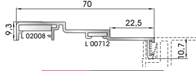
Additional profile for casing trim 82422
