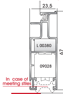
29035 W=699gr/m A=0,335m 2 /m Insect screen sash for 29005 & 29015 profiles
