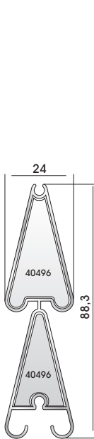
Hooked casing trim "Curve"
