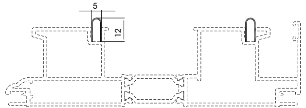
94235 W=134gr/m A=0,050m 2 /m Stainless track insert (for window/shutter/insect screen)
