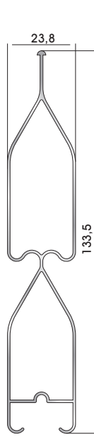
Shutter louver 'canted'
