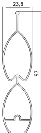
Shutter louver 'round'
