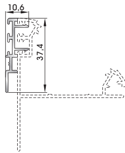
Additional profile for casing trim 82422
