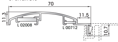
Casing trim for built-in windows/balcony doors & shutters
