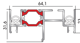
15045 W=945gr/m A=0,391m 2 /m Additional profile (for 15025 window/balcony door sash) (meeting stiles)
