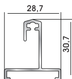
29005 W=294gr/m A=0,169m 2 /m Insect screen single track
