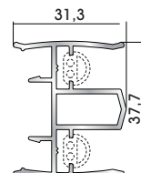
94052 W=574gr/m A=0,280m 2 /m Additional profile (for 94505, insect screen sash profile)
