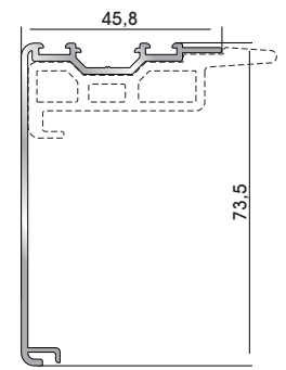
15035 W=566gr/m A=0,295m 2 /m Hook (for 15025 window/balcony door sash)
