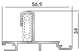
94105 W=516gr/m A=0,271m 2 /m Additional track
