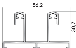
29015 W=570gr/m A=0,325m 2 /m Insect screen double track
