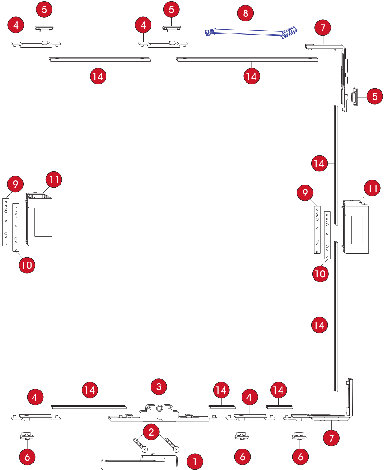
Mechanism for pivot one leaf windows
