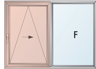
Mechanism for tilt & slide first leaf of two leaves windows
