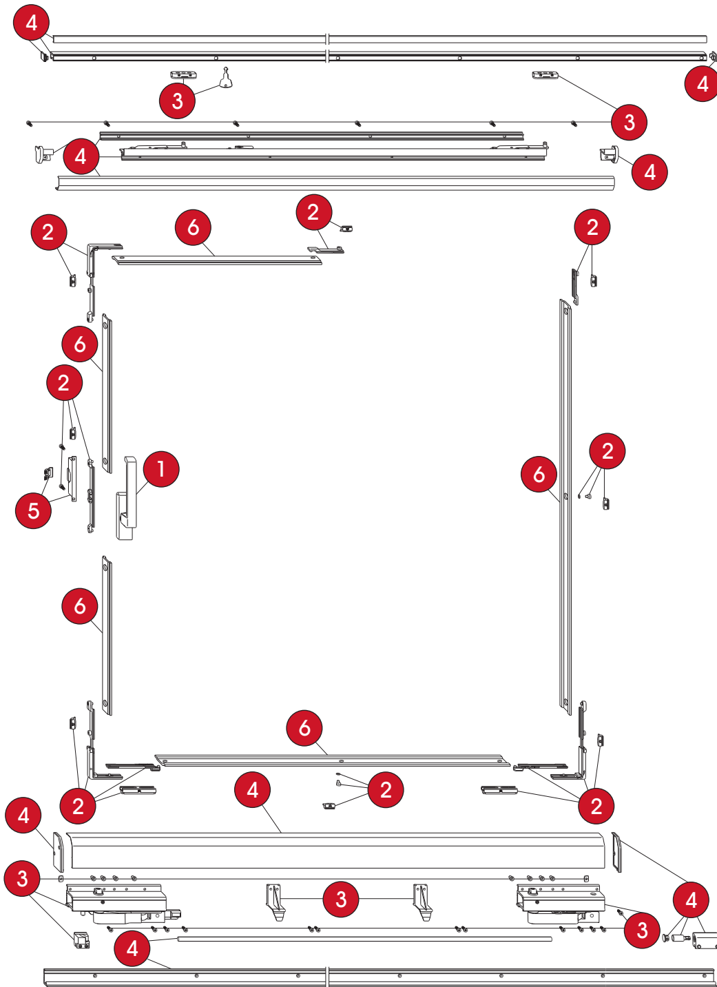
Mechanism for tilt & slide first leaf of two leaves windows
