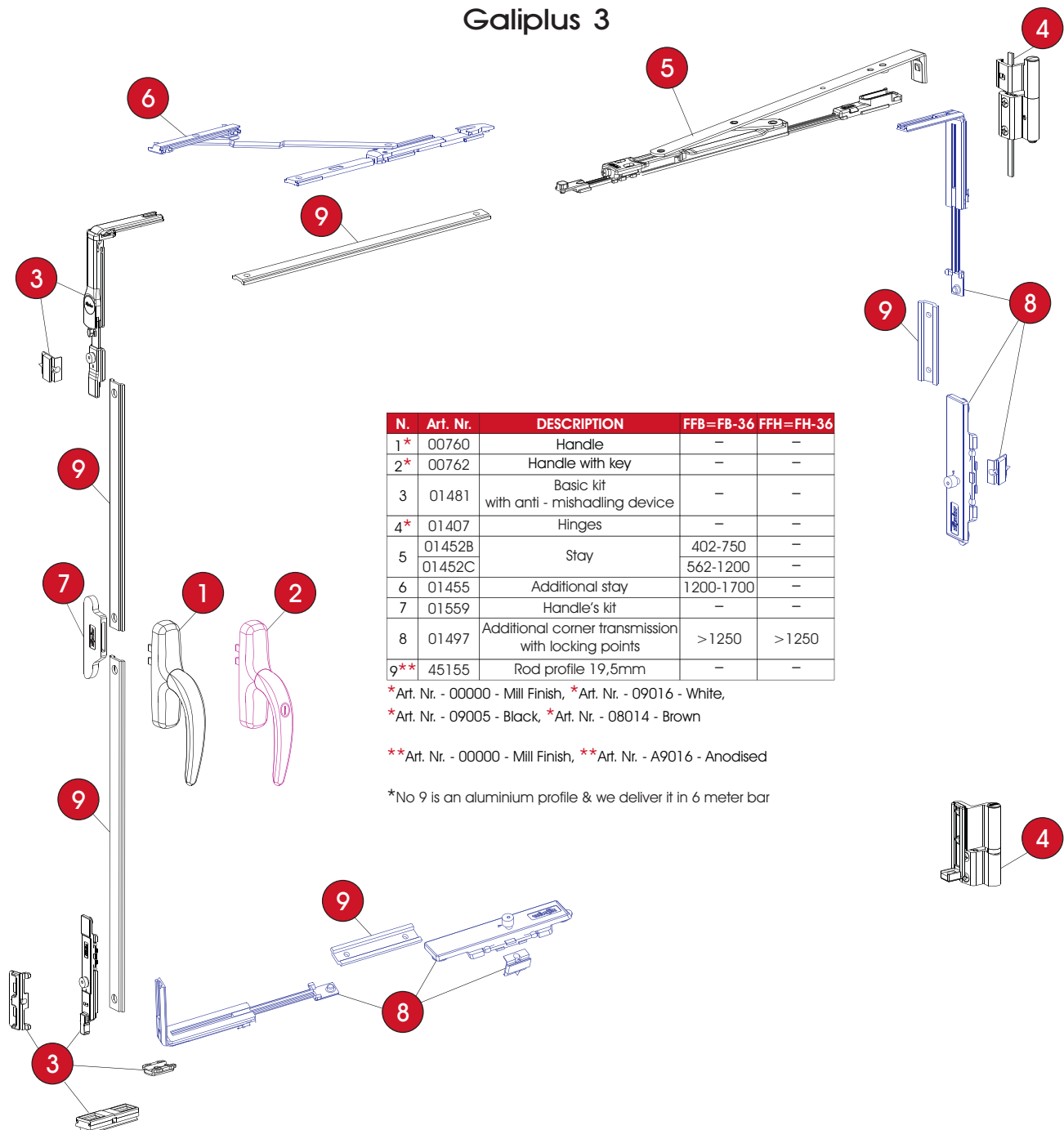
Mechanism for tilt & turn - one leaf - windows & doors
