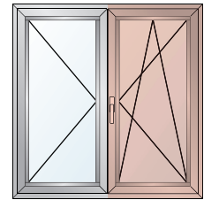
Mechanism for tilt & turn - first leaf of two leaves - windows & doors
